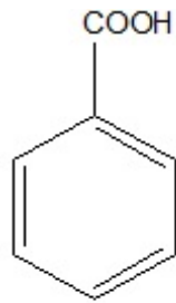
Benzoic Acid
